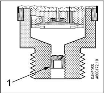
1 Pulse-snubber
